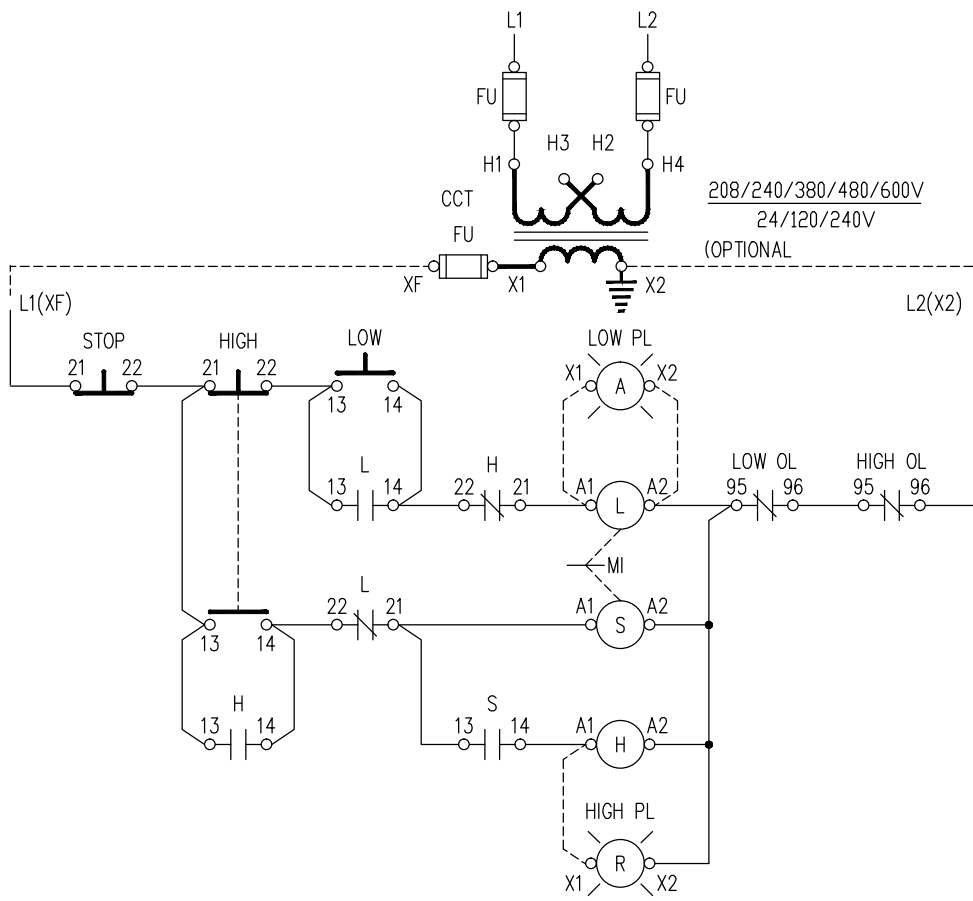
STOP - LOW - HIGH PUSHBUTTON
