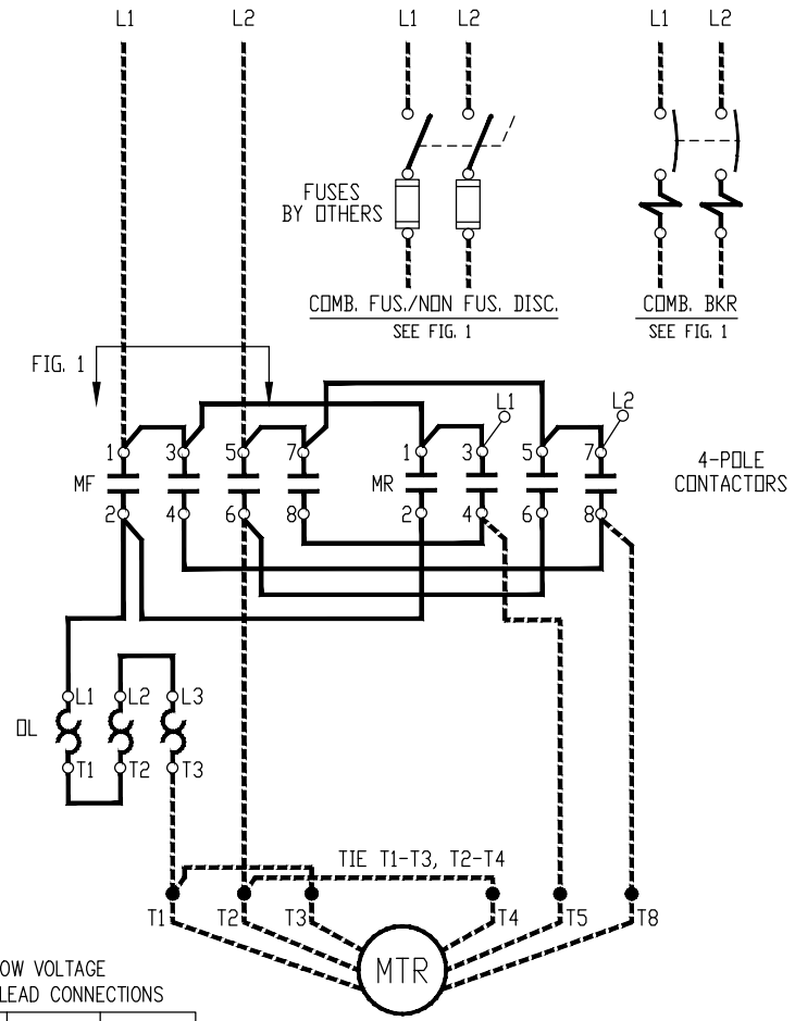
1-PH REVERSING 6-LEAD CAPACITOR START MOTOR
