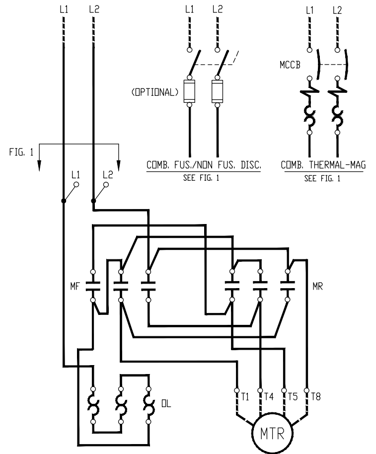
1-PH 4-LEAD CAPACITOR OR SPLIT PHASE MOTOR
