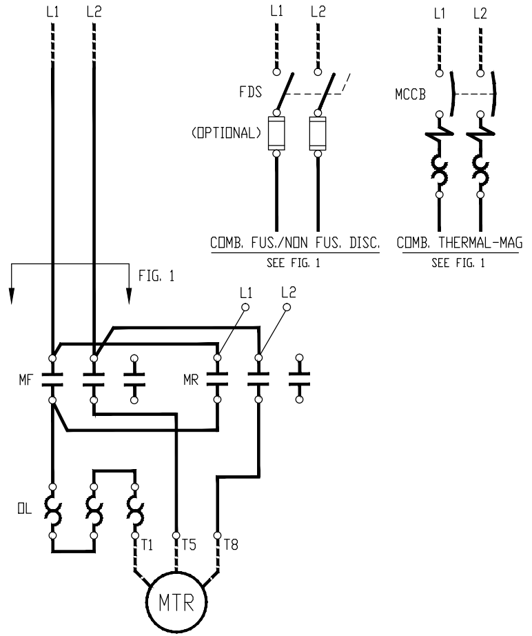
1-PH 3-LEAD REPULSION INDUCTION MOTOR
