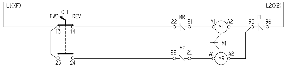
FORWARD OFF REVERSE SEL. SW.
