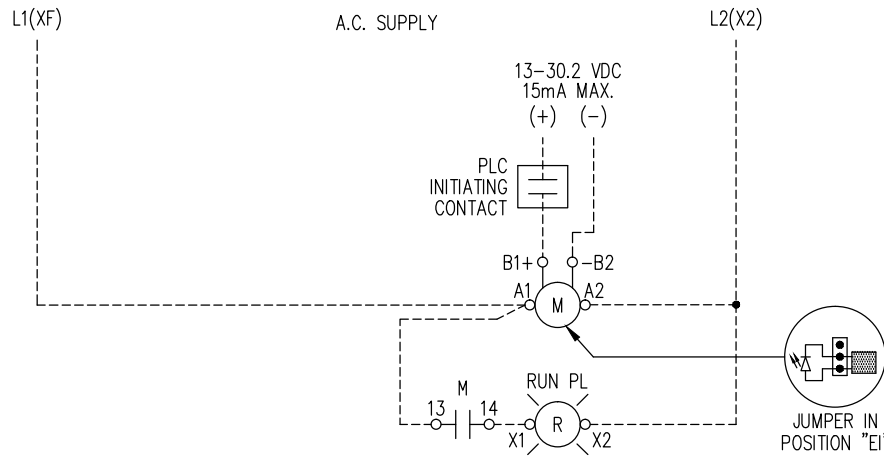
"EI" MODE OR INTERFACE OPERATION
