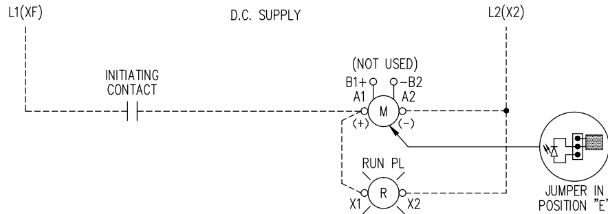
"E" MODE OR NORMAL OPERATION
