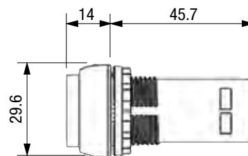
Momentary Pushbutton Device Extended (D7D-E)
