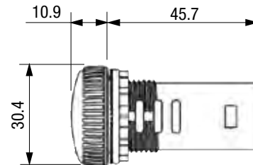
Pilot Light Devices (D7D-P)
