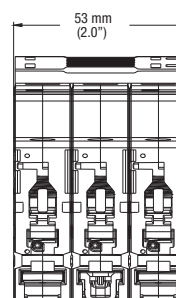
3-Pole
