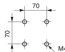
Drill Plan (base)
