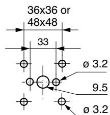
Drill Plan (operator)
