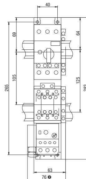
KTB7-45H + CA7-43 + CEP7-E
