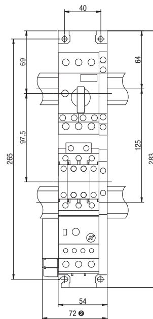
KTB7-25H + CA7-30...37 + CEP7-D/E
