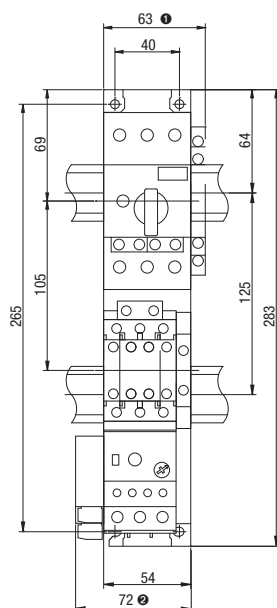
KTB7-45H + CA7-30...37 + CEP7-D/E
