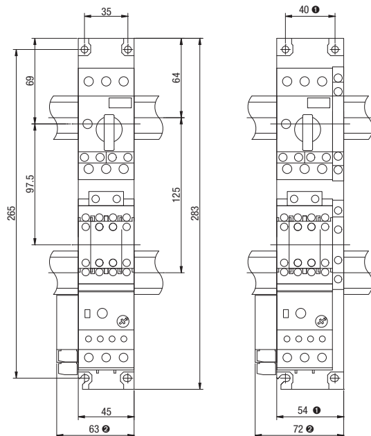
KTB7-45H + CA7-30...37 + CEP7-D/E
