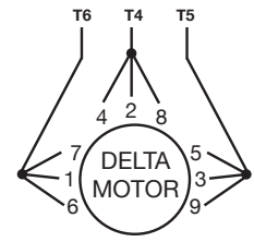
9 LEAD, 230V LOW VOLTAGE, MOTOR CONNECTIONS
